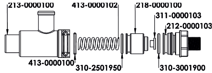
YP-71/81 EMNİYET VALFİ PATLATILMIŞ MODEL SAFETY VALVE PART DIAGRAM
