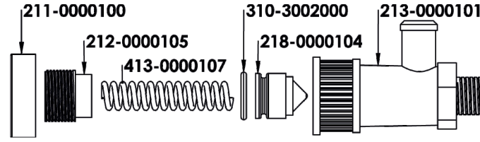
YP-70/80 EMNİYET VALFİ PATLATILMIŞ MODEL SAFETY VALVE PART DIAGRAM
